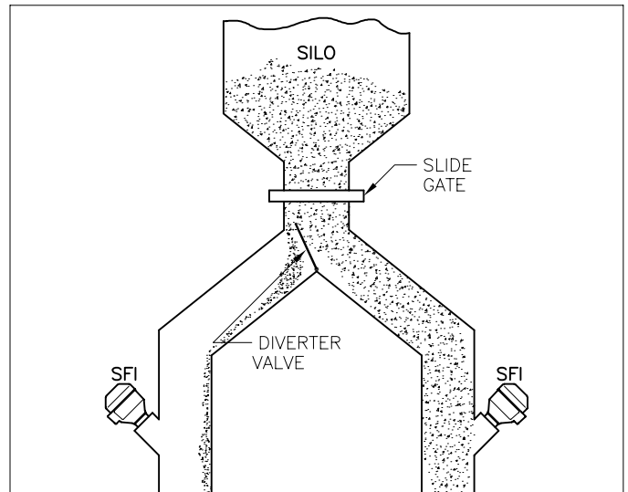
SFI signals underfeed or overfeed conditions that may result from malfunctioning process equipment such as a diverter valve.
