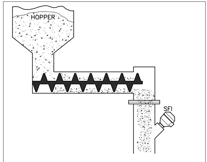
SFI provides mass flow indication to help ensure flow rate from feeders and conveyors is within acceptable range.
